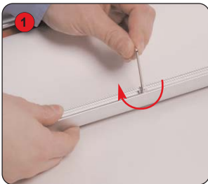
1 Loosen the Top grip rail screws using a 2.5mm allen key.
