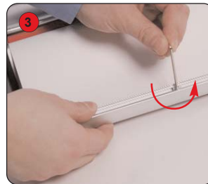
3 Tighten the Top grip rail screws.
